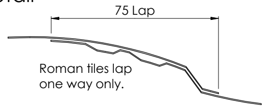
Figure 3.4 Lap Section
