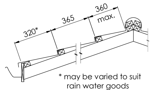
Figure 3.5 Batten Layout
