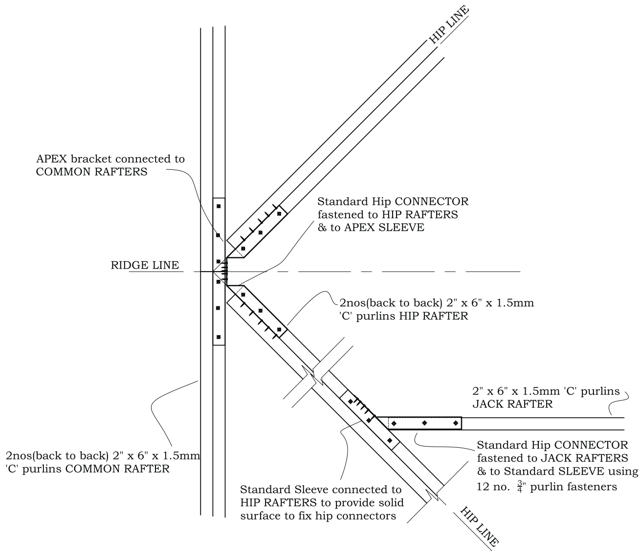
Typical HIP Rafter Detail
