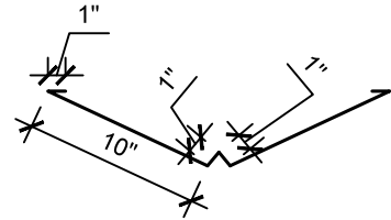
24" Valley
