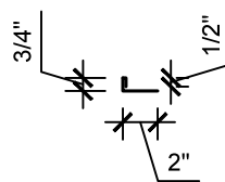
4" Angle Cleat
