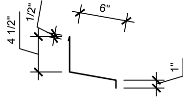
12" Head Wall
