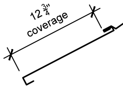
Bermuda Panel
