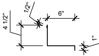
12" Side Wall
