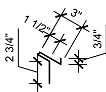
8" Starter
