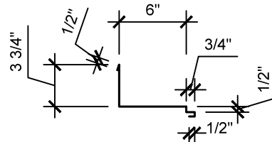
12" Side Wall
