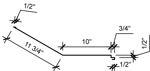
24" Transition
