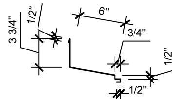
12" Head Wall
