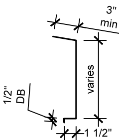
18" Fascia
