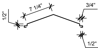
18" Ridge / Hip
