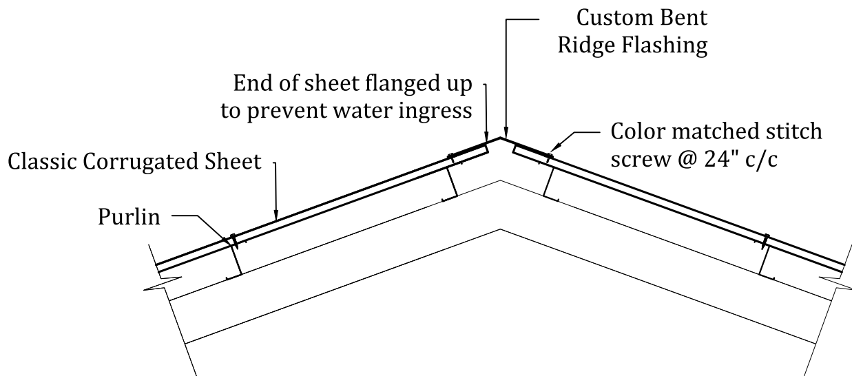
RIDGE - TYPICAL
