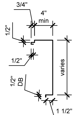
24" Gable
