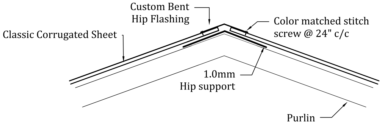
Hip- TYPICAL
