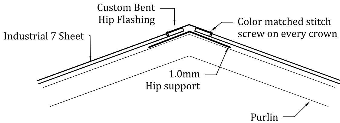
Hip- TYPICAL
