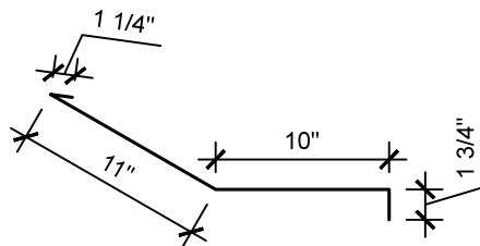
24" Transition
