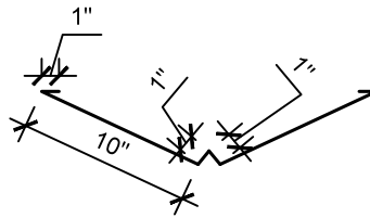
24" Valley
