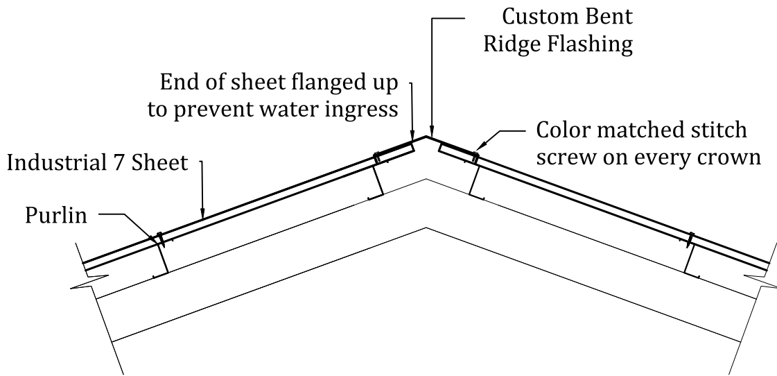
RIDGE - TYPICAL
