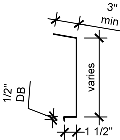
18" Fascia
