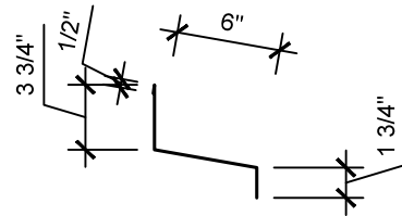
12" Head Wall
