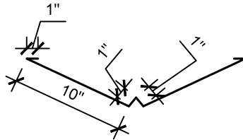
24" Valley
