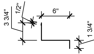
12" Side Wall
