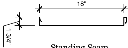
Standing Seam
