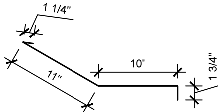
24" Transition
