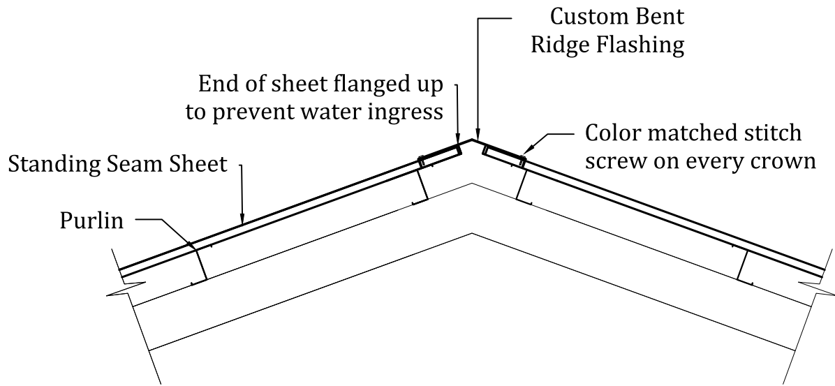
RIDGE - TYPICAL
