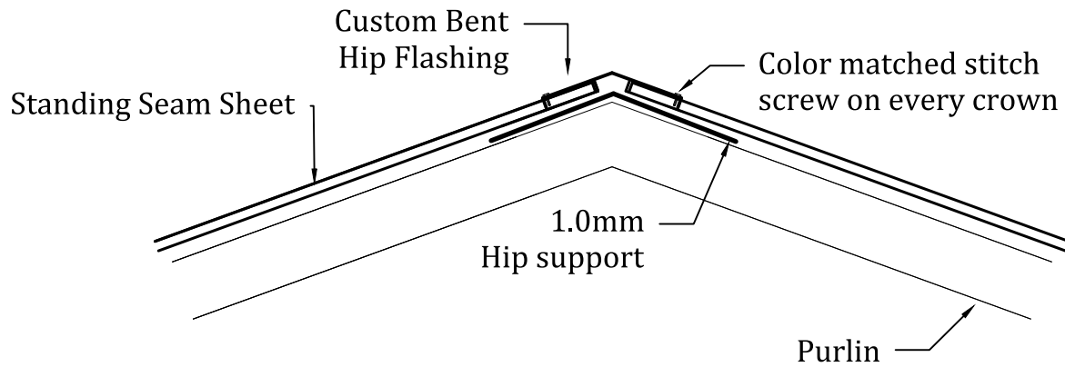
Hip- TYPICAL
